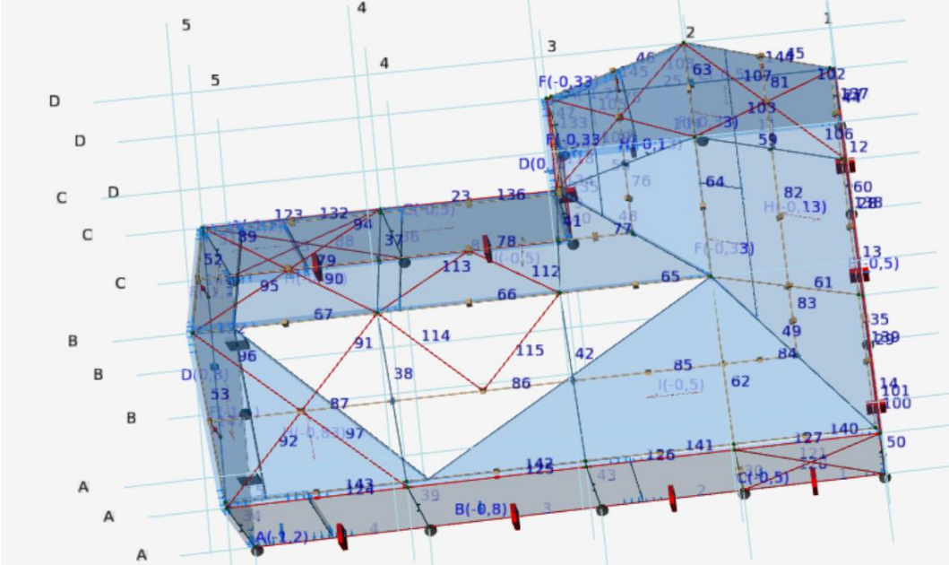
Belastingsgeval 521 Wind -Y A
